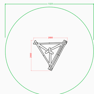
Plan elevation
