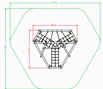
Plan elevation
