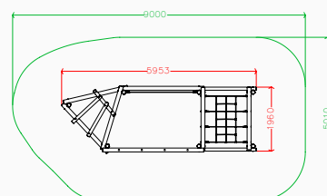
Plan elevation
