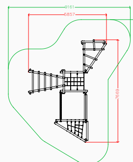
Plan elevation
