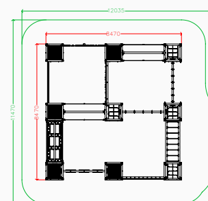
Plan elevation
