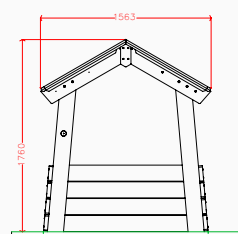
Side elevation
