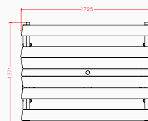
Plan elevation
