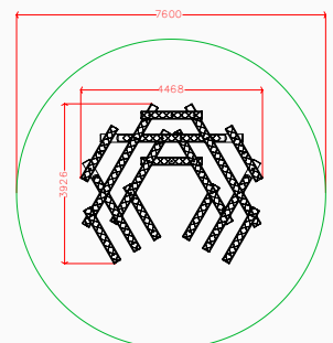
Plan elevation
