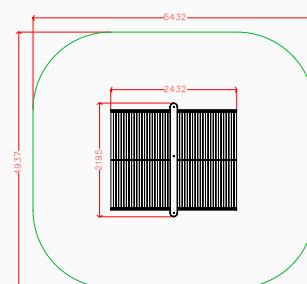
Plan elevation
