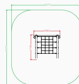
Plan elevation
