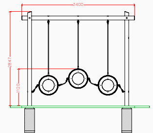
Plan elevation
