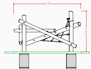
Side elevation
