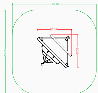
Plan elevation
