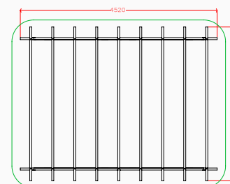
Plan elevation
