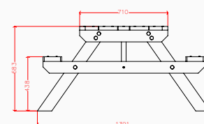
Side elevation
