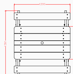
Plan elevation
