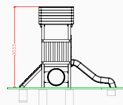
Side elevation
