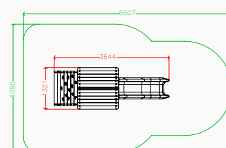
Plan elevation
