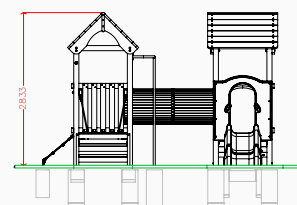
Side elevation
