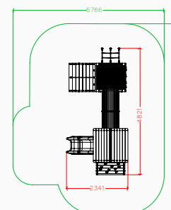
Plan elevation
