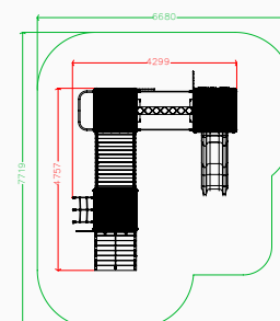
Plan elevation
