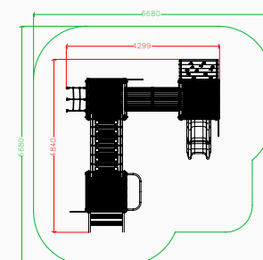
Plan elevation
