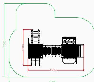
Plan elevation
