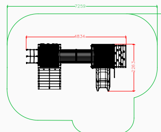
Plan elevation
