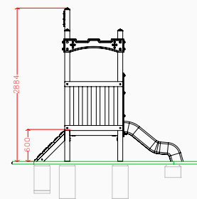
Plan elevation
