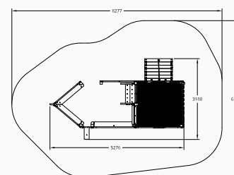
Plan elevation
