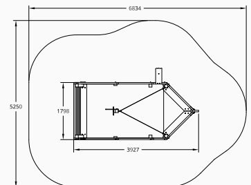
Plan elevation
