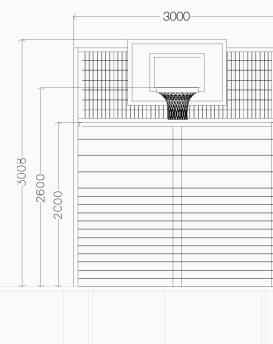
Plan elevation
