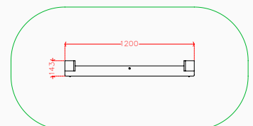
Plan elevation
