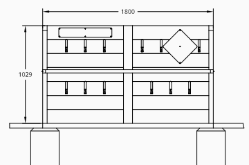
Plan elevation
