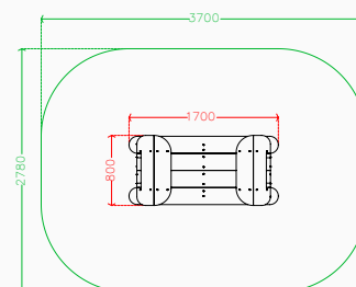
Plan elevation
