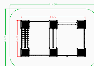
Plan elevation
