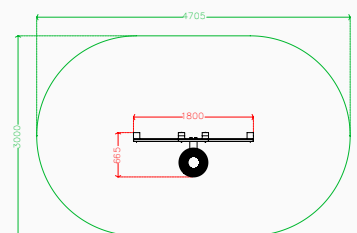
Plan elevation
