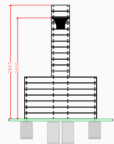
Plan elevation
