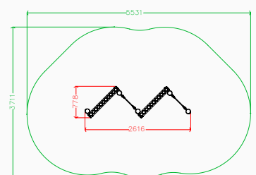
Plan elevation
