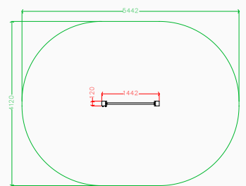
Plan elevation
