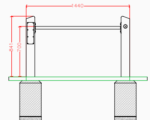
Plan elevation
