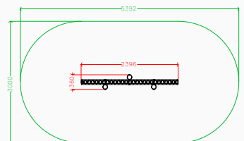
Plan elevation
