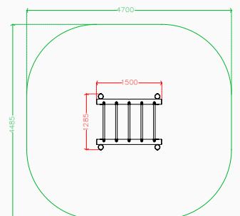
Plan elevation
