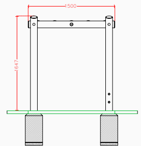
Side elevation
