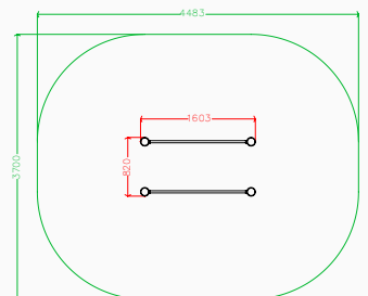
Plan elevation
