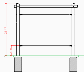
Plan elevation
