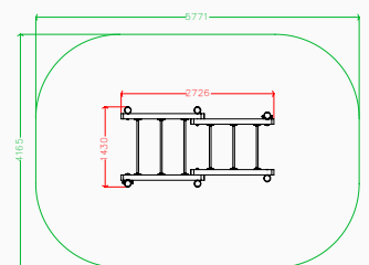
Plan elevation
