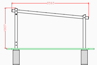
Side elevation
