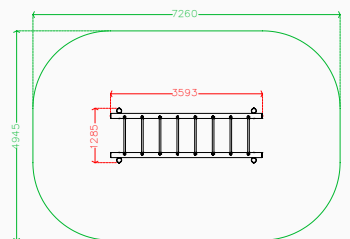
Plan elevation
