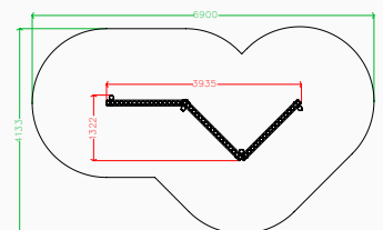
Plan elevation
