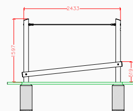
Side elevation
