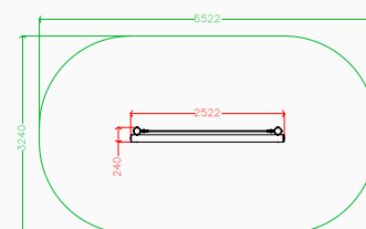
Plan elevation
