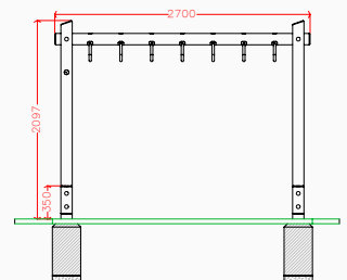
Plan elevation
