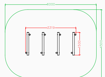
Plan elevation
