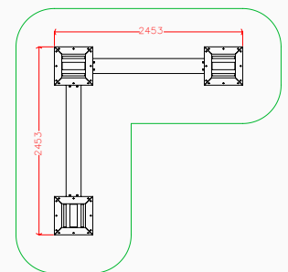
Plan elevation
