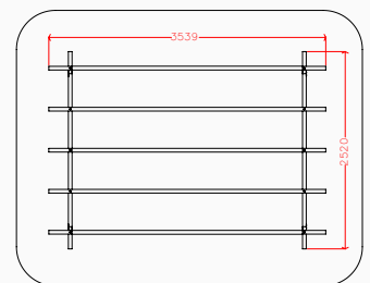
Plan elevation
